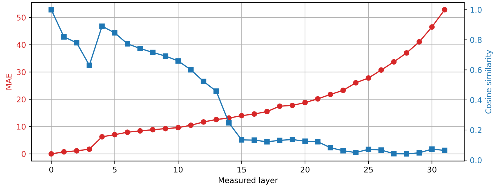
SmolLM2-360M | Prompt 1 Spared layer 18 | Hybrid vs unquantized
