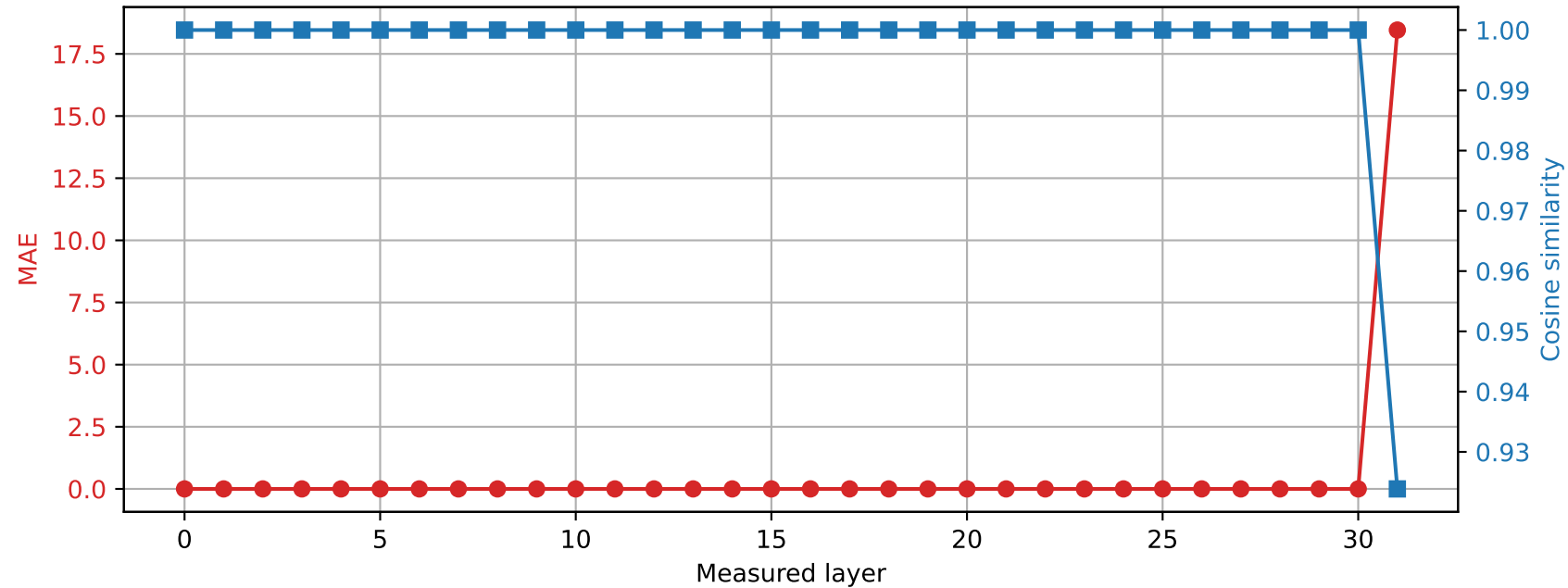
SmolLM2-360M | Prompt 1 Spared layer 30 | Hybrid vs quantized
