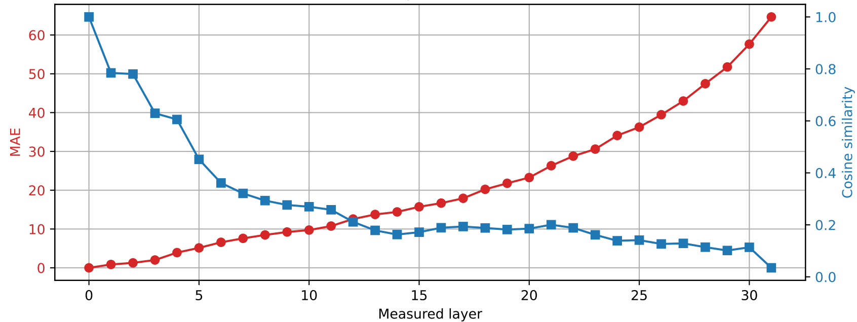
SmolLM2-360M | Prompt 2 Spared layer 0 | Hybrid vs quantized
