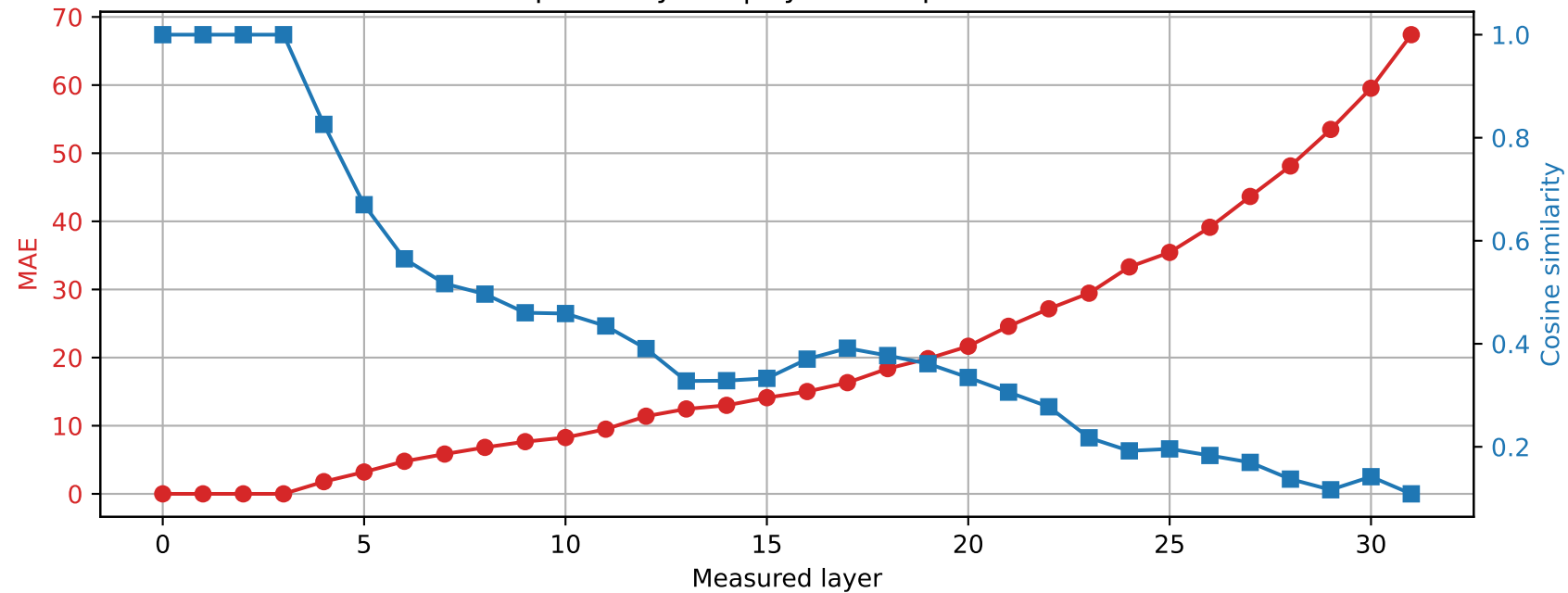
SmolLM2-360M | Prompt 2 Spared layer 3 | Hybrid vs quantized
