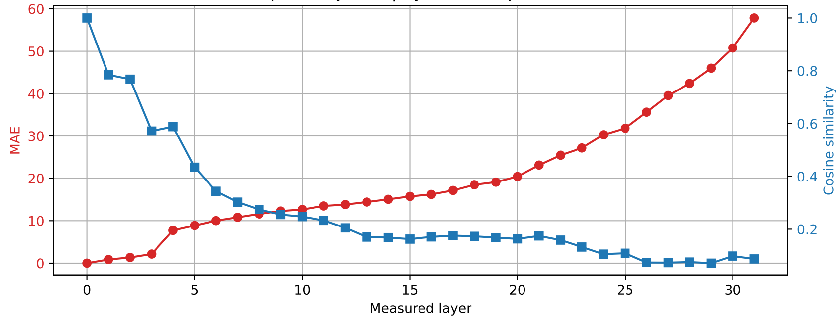
SmolLM2-360M | Prompt 2 Spared layer 11 | Hybrid vs unquantized
