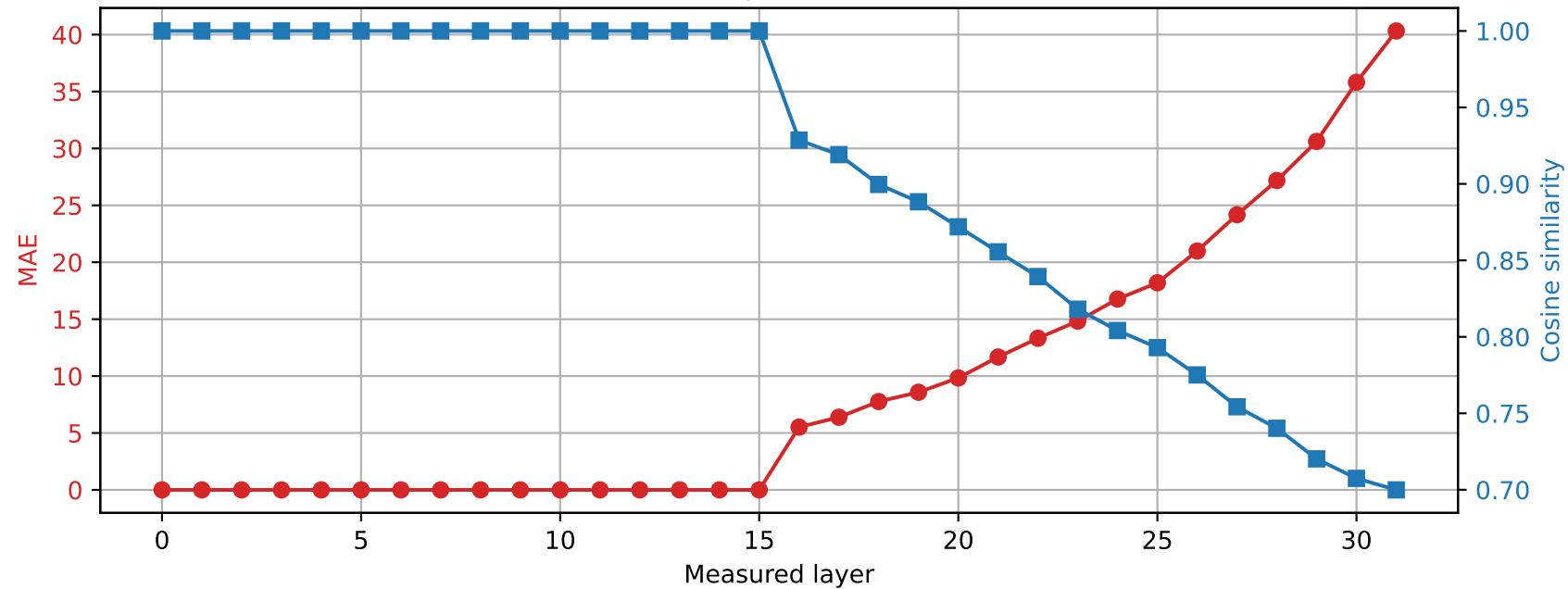
SmolLM2-360M | Prompt 2 Spared layer 15 | Hybrid vs quantized
