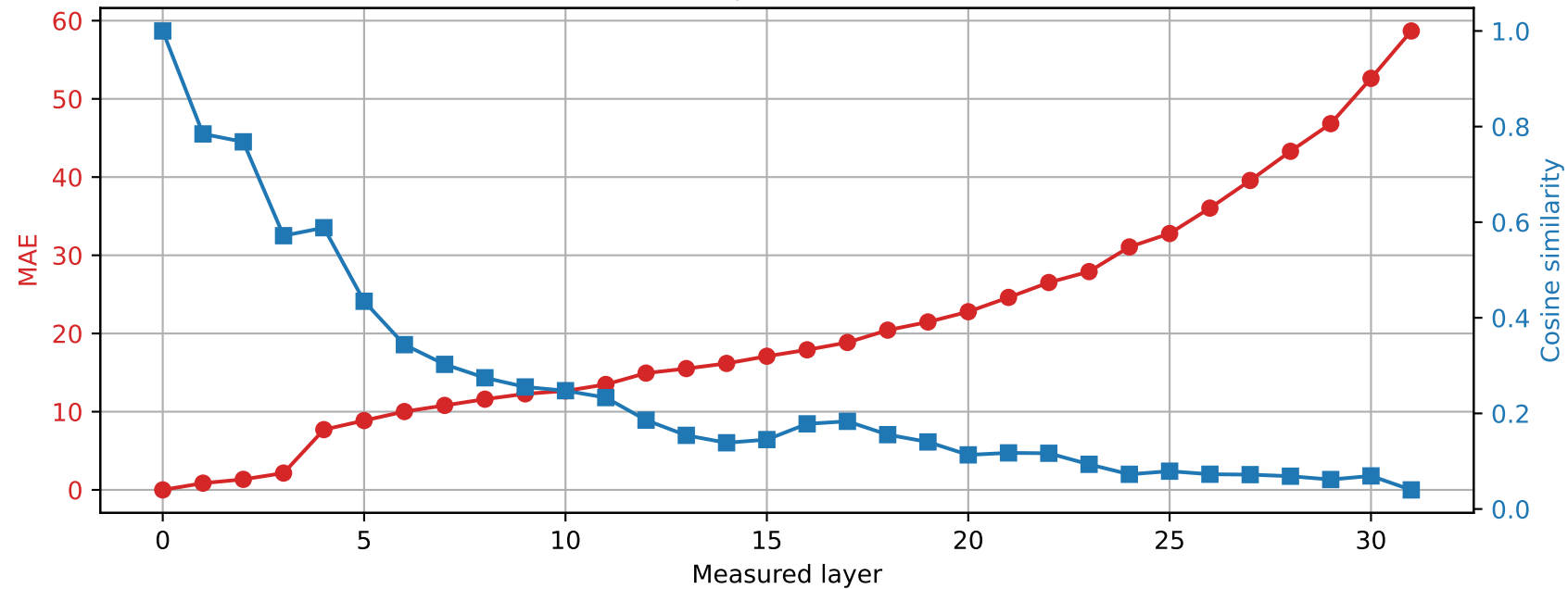
SmolLM2-360M | Prompt 2 Spared layer 15 | Hybrid vs unquantized
