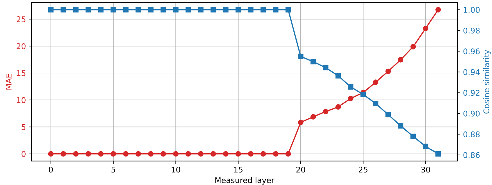
SmolLM2-360M | Prompt 2 Spared layer 19 | Hybrid vs quantized
