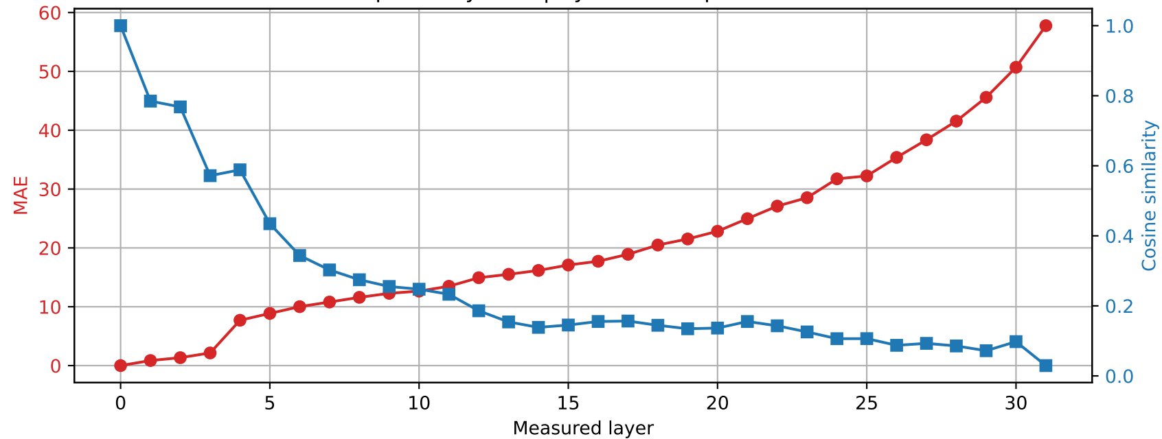
SmolLM2-360M | Prompt 2 Spared layer 24 | Hybrid vs unquantized
