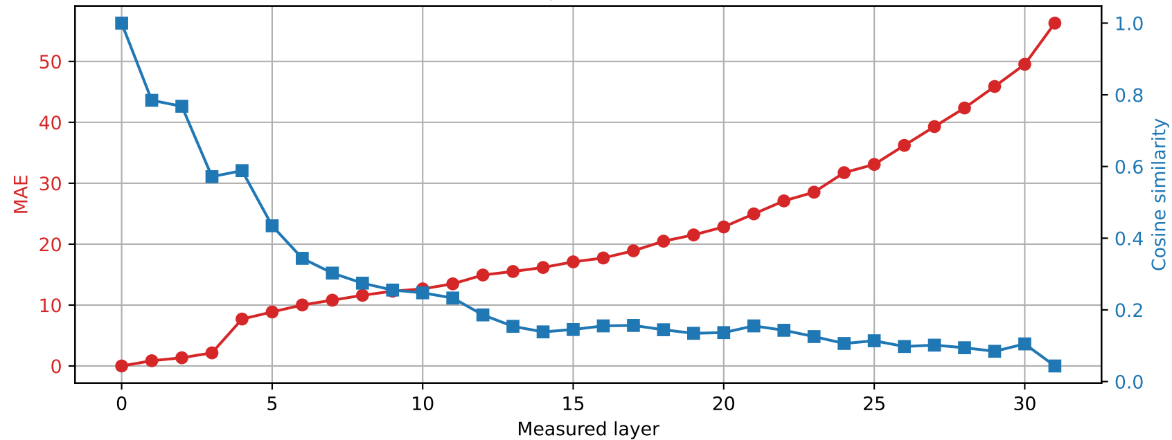
SmolLM2-360M | Prompt 2 Spared layer 29 | Hybrid vs unquantized
