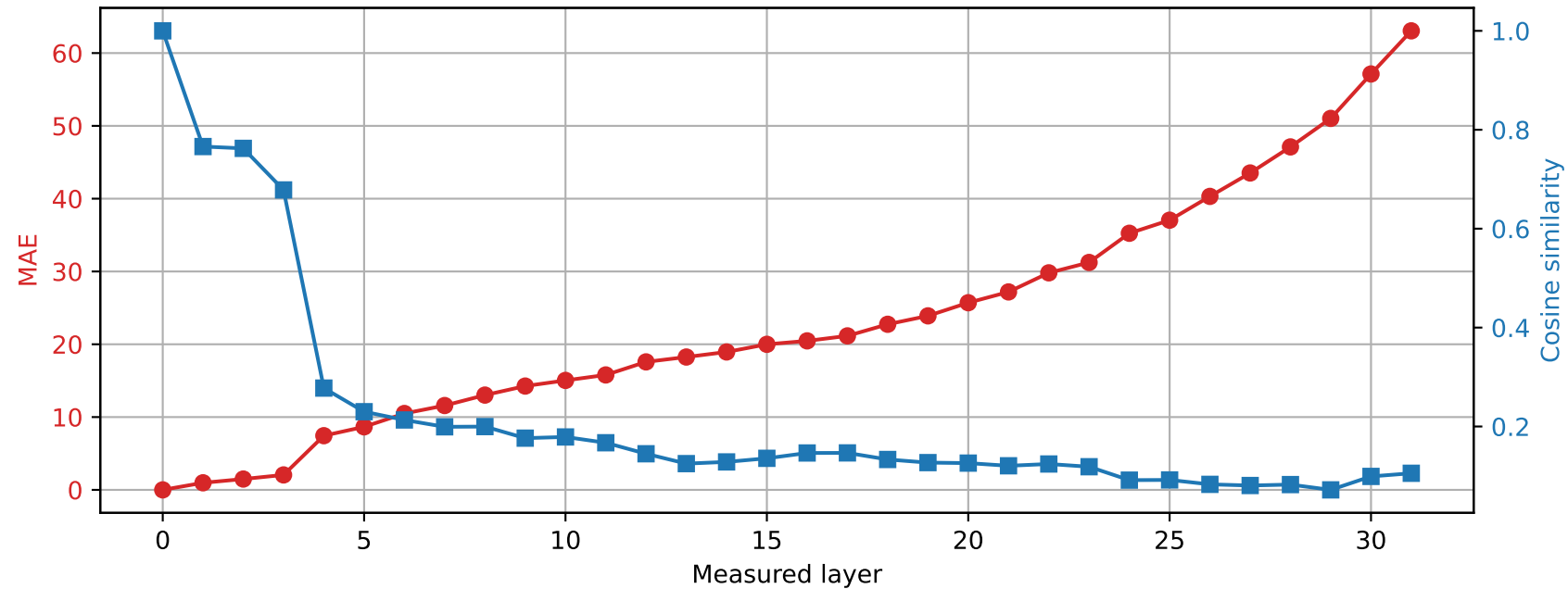
SmolLM2-360M | Prompt 3 Unquantized vs quantized int4
