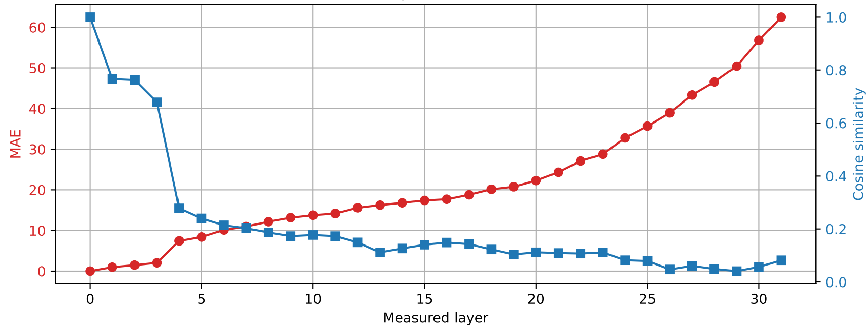
SmolLM2-360M | Prompt 3 Spared layer 4 | Hybrid vs unquantized
