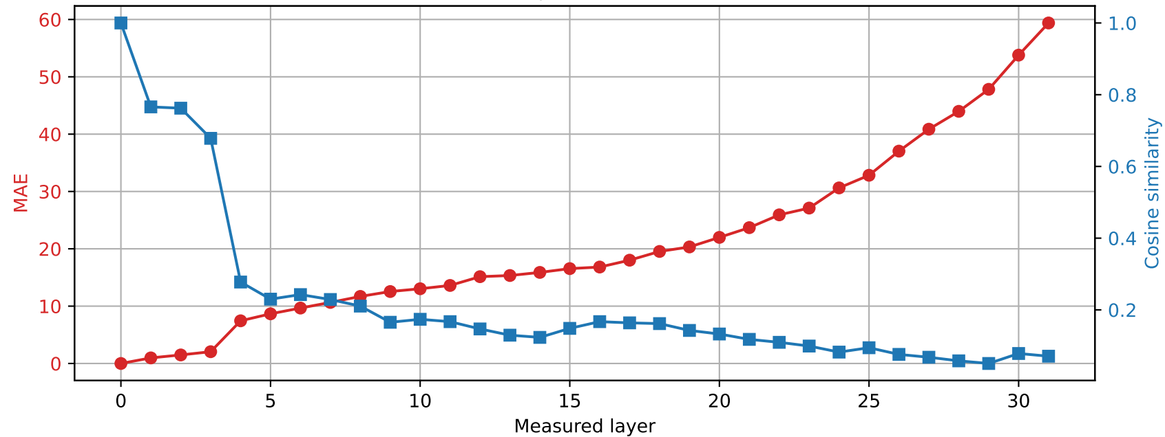
SmolLM2-360M | Prompt 3 Spared layer 5 | Hybrid vs unquantized
