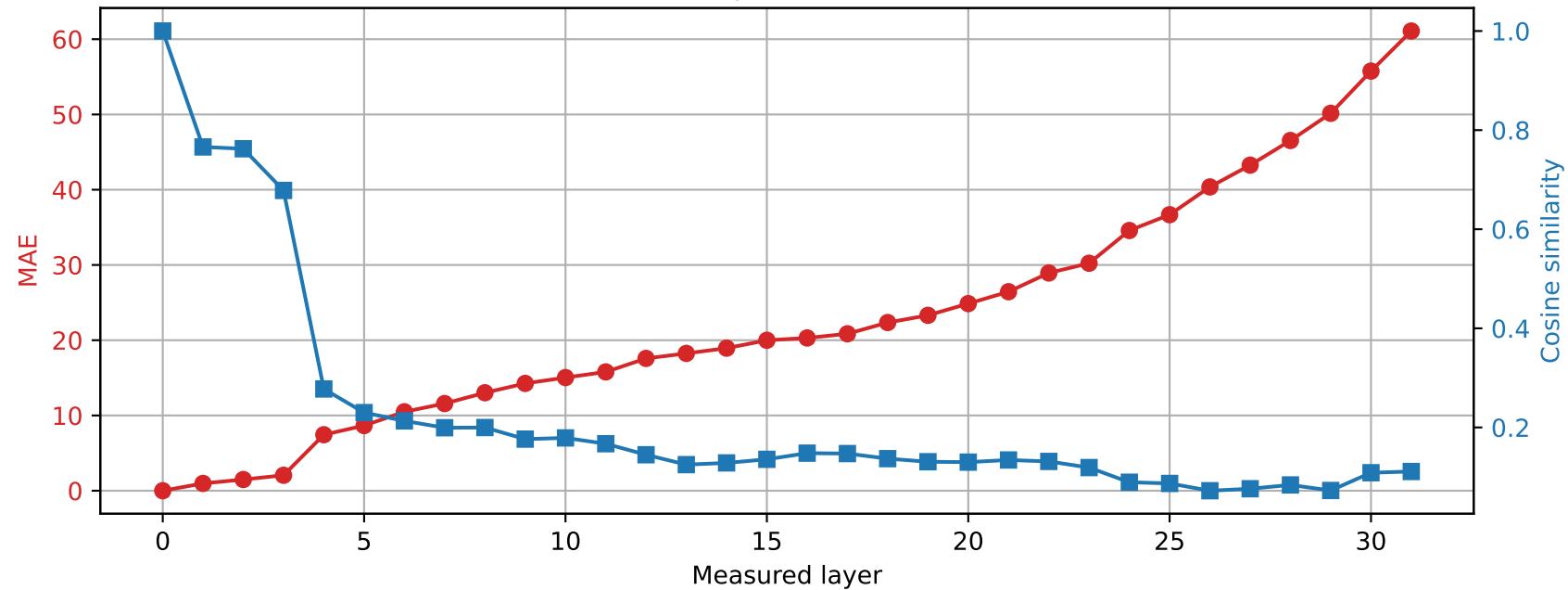
SmolLM2-360M | Prompt 3 Spared layer 15 | Hybrid vs unquantized
