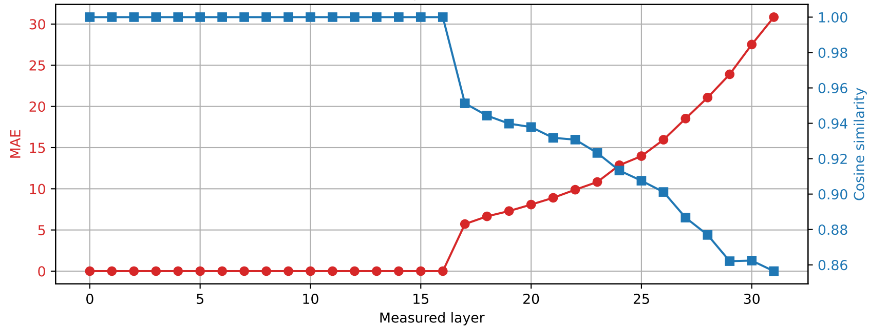
SmolLM2-360M | Prompt 3 Spared layer 16 | Hybrid vs quantized
