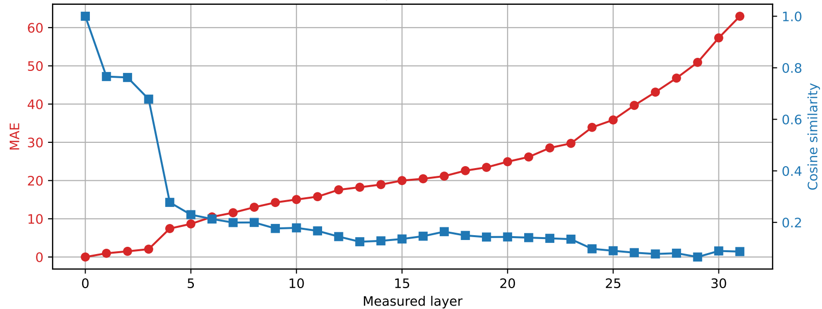
SmolLM2-360M | Prompt 3 Spared layer 16 | Hybrid vs unquantized
