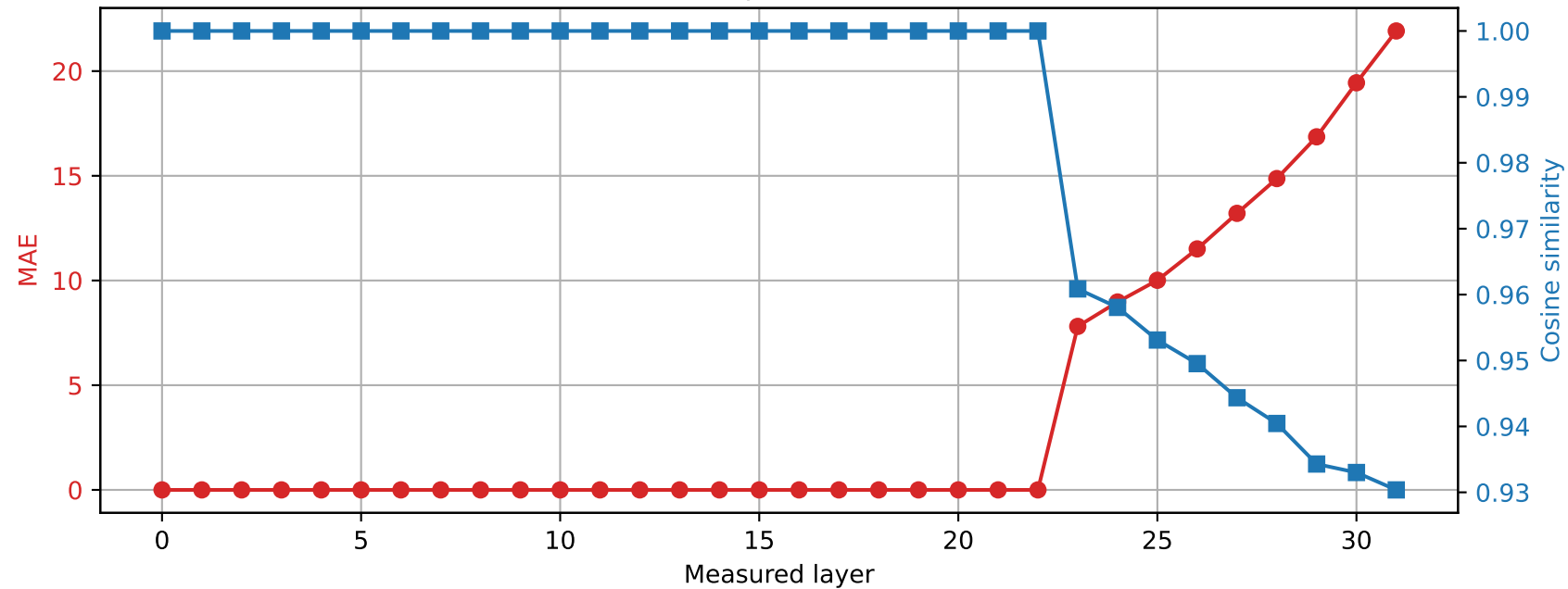
SmolLM2-360M | Prompt 3 Spared layer 22 | Hybrid vs quantized
