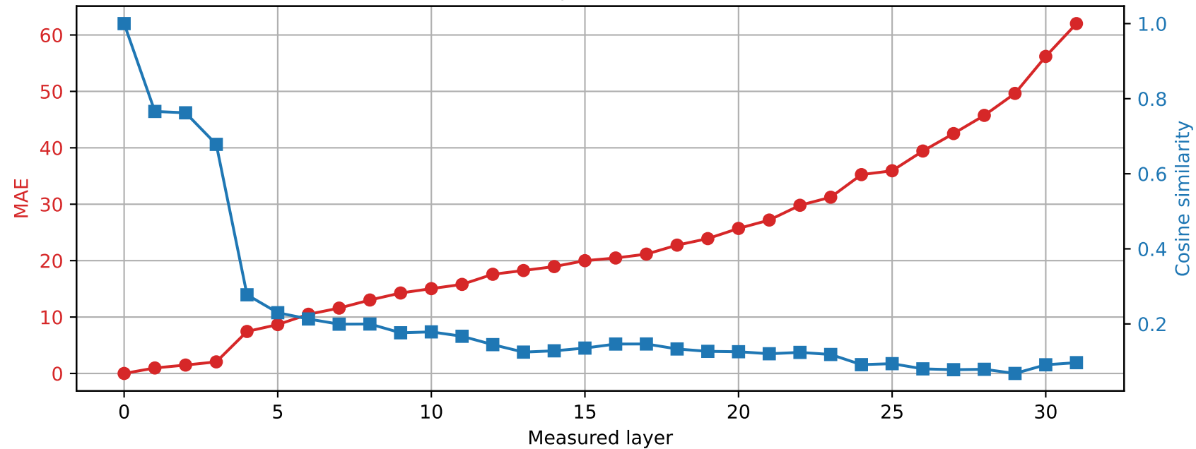
SmolLM2-360M | Prompt 3 Spared layer 24 | Hybrid vs unquantized
