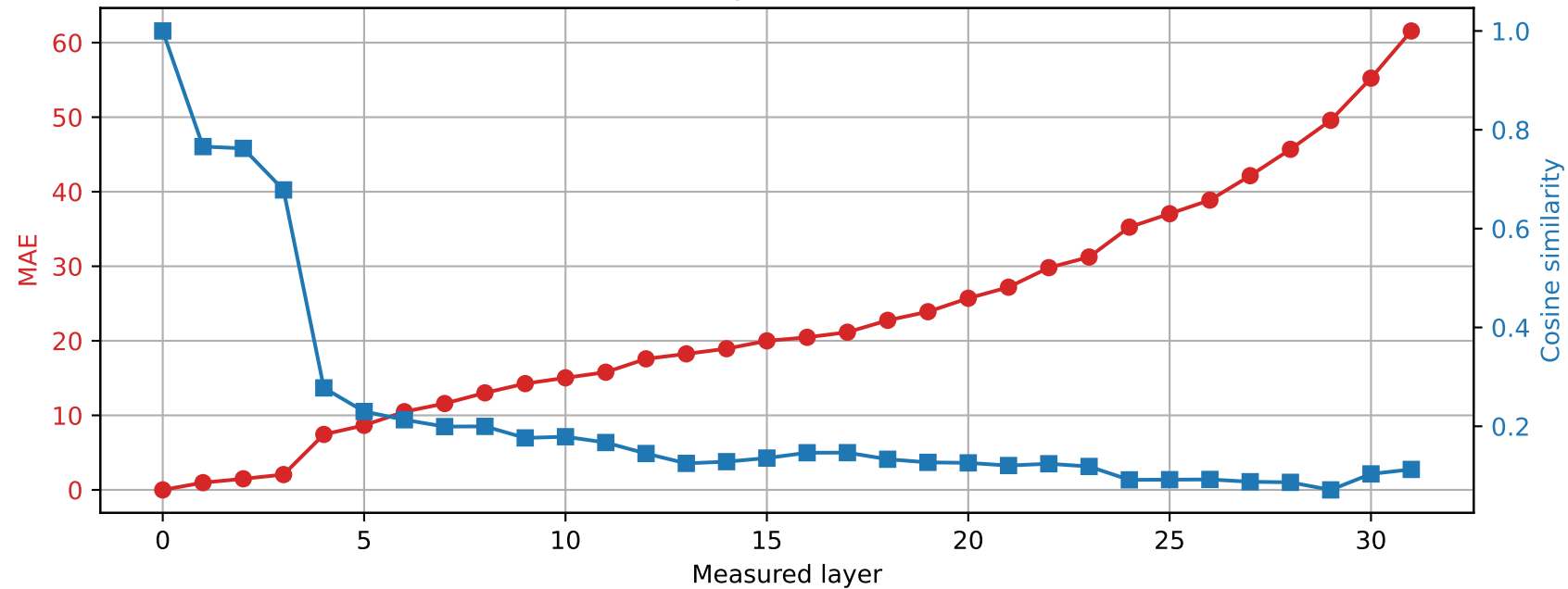
SmolLM2-360M | Prompt 3 Spared layer 25 | Hybrid vs unquantized
