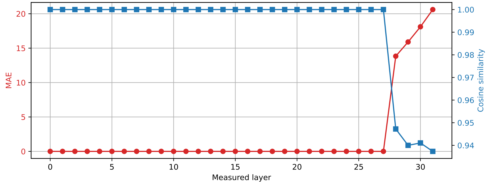
SmolLM2-360M | Prompt 3 Spared layer 27 | Hybrid vs quantized
