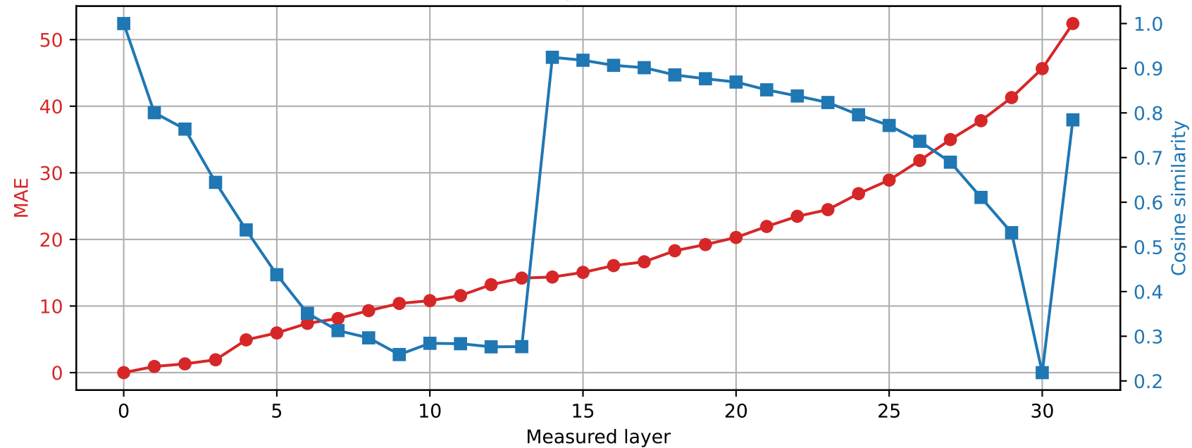
SmolLM2-360M | Prompt 4 Spared layer 0 | Hybrid vs quantized
