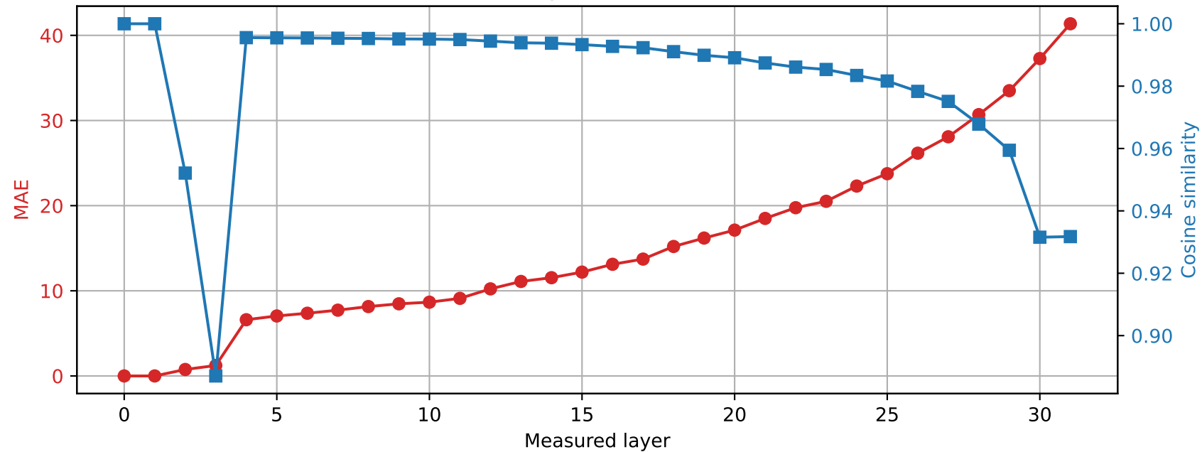
SmolLM2-360M | Prompt 4 Spared layer 0 | Hybrid vs unquantized
