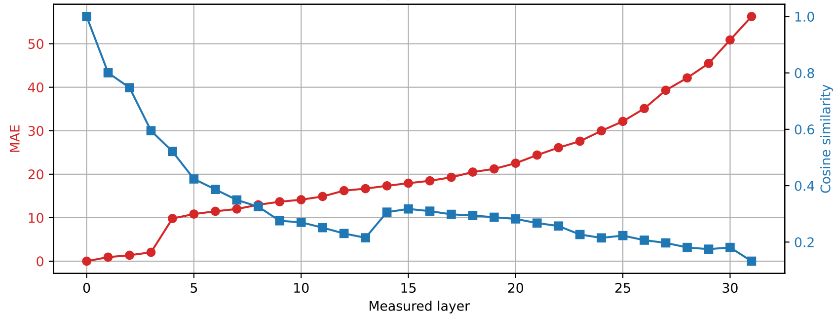
SmolLM2-360M | Prompt 4 Spared layer 5 | Hybrid vs unquantized
