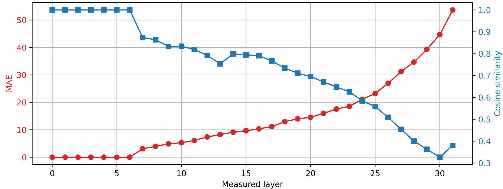
SmolLM2-360M | Prompt 4 Spared layer 6 | Hybrid vs quantized
