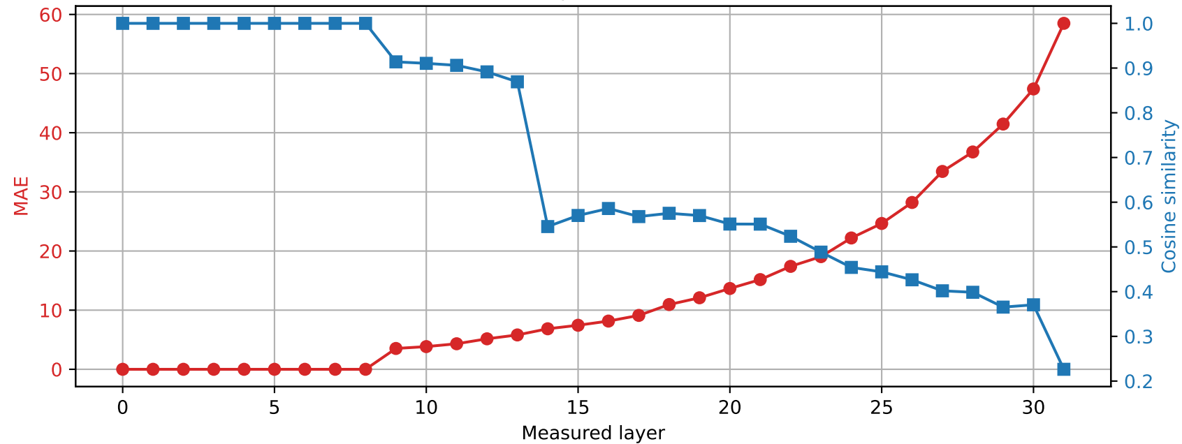
SmolLM2-360M | Prompt 4 Spared layer 8 | Hybrid vs quantized
