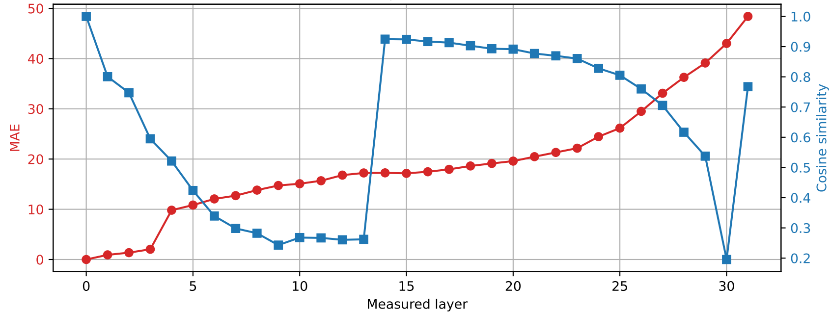
SmolLM2-360M | Prompt 4 Spared layer 14 | Hybrid vs unquantized
