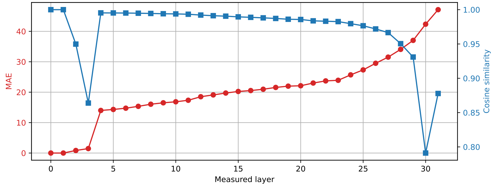
SmolLM2-360M | Prompt 0 Spared layer 0 | Hybrid vs unquantized
