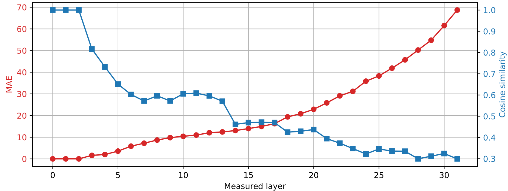
SmolLM2-360M | Prompt 0 Spared layer 2 | Hybrid vs quantized
