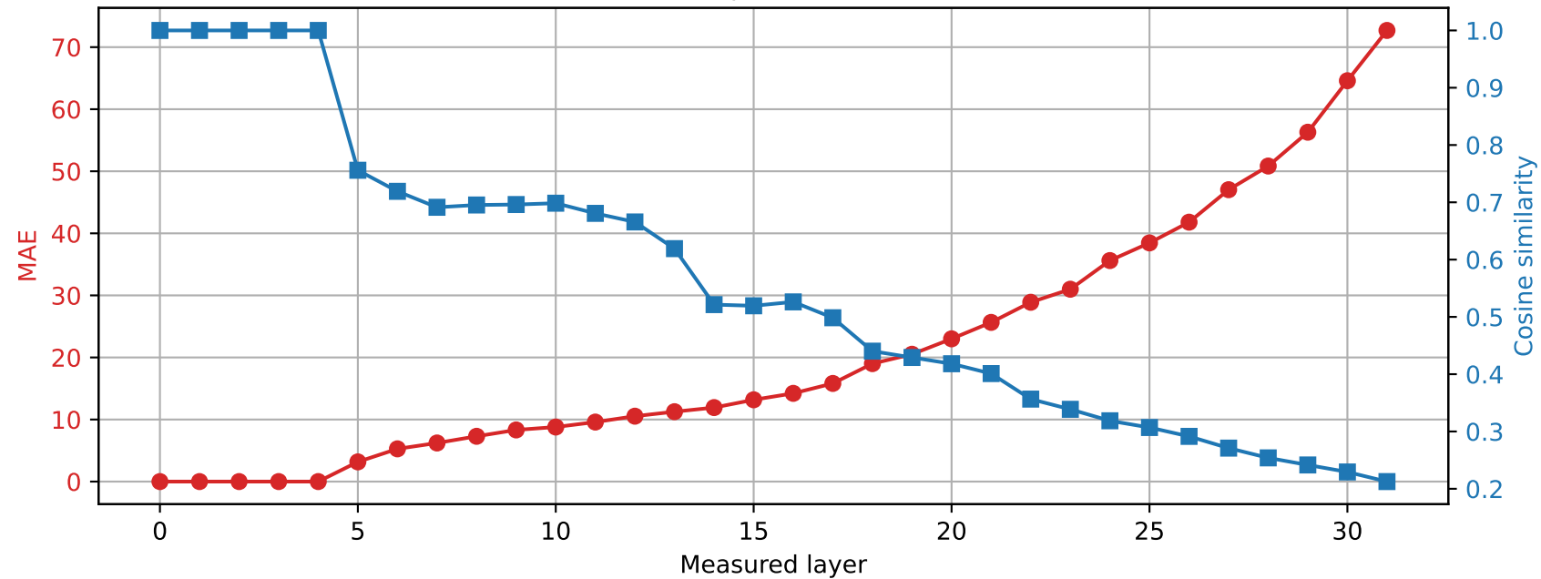
SmolLM2-360M | Prompt 0 Spared layer 4 | Hybrid vs quantized
