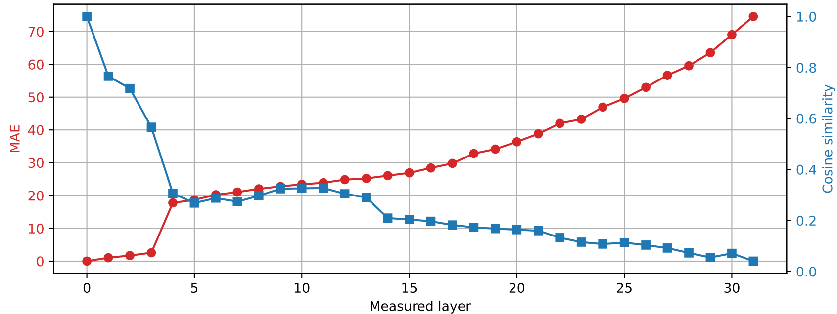
SmolLM2-360M | Prompt 0 Spared layer 13 | Hybrid vs unquantized
