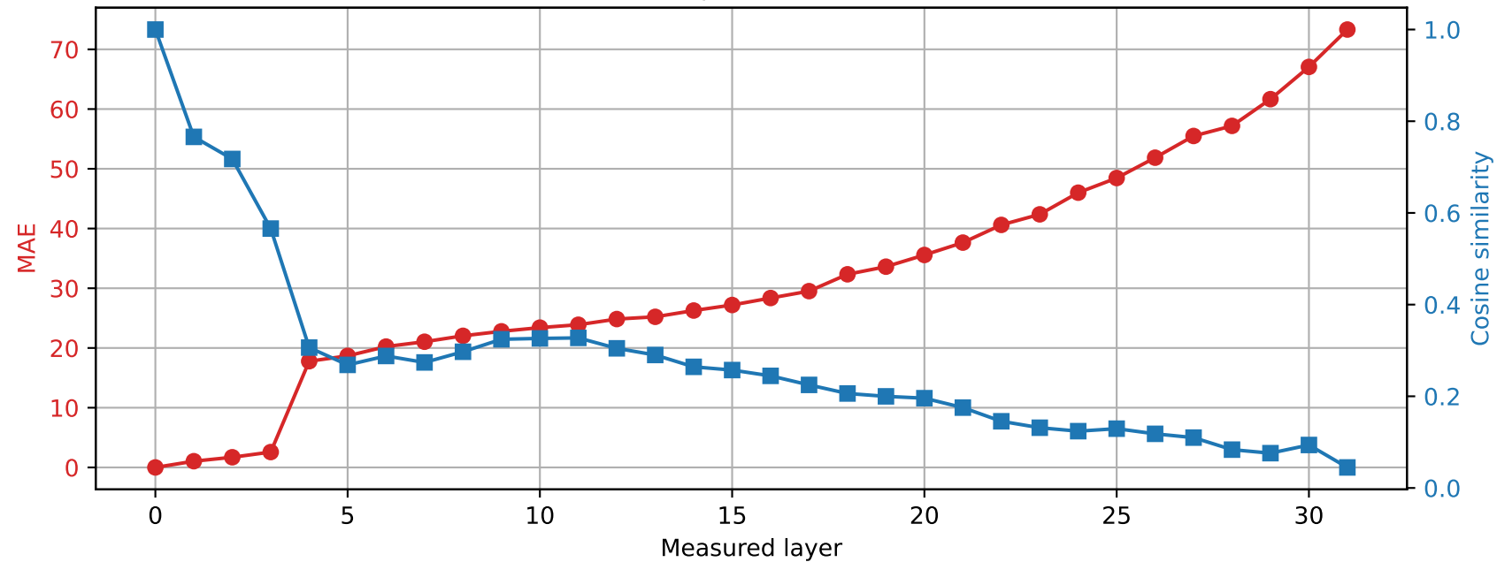
SmolLM2-360M | Prompt 0 Spared layer 27 | Hybrid vs unquantized
