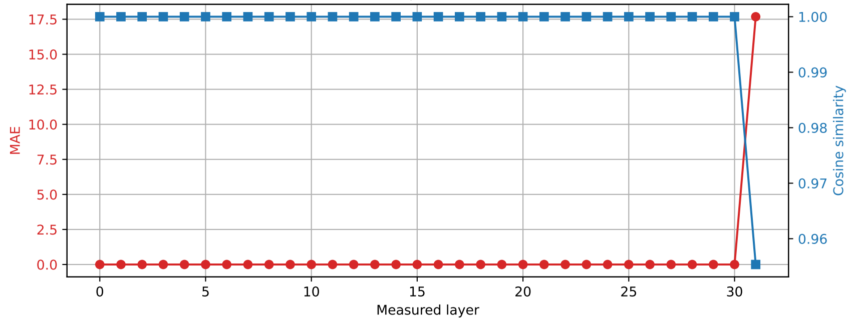
SmolLM2-360M | Prompt 0 Spared layer 30 | Hybrid vs quantized
