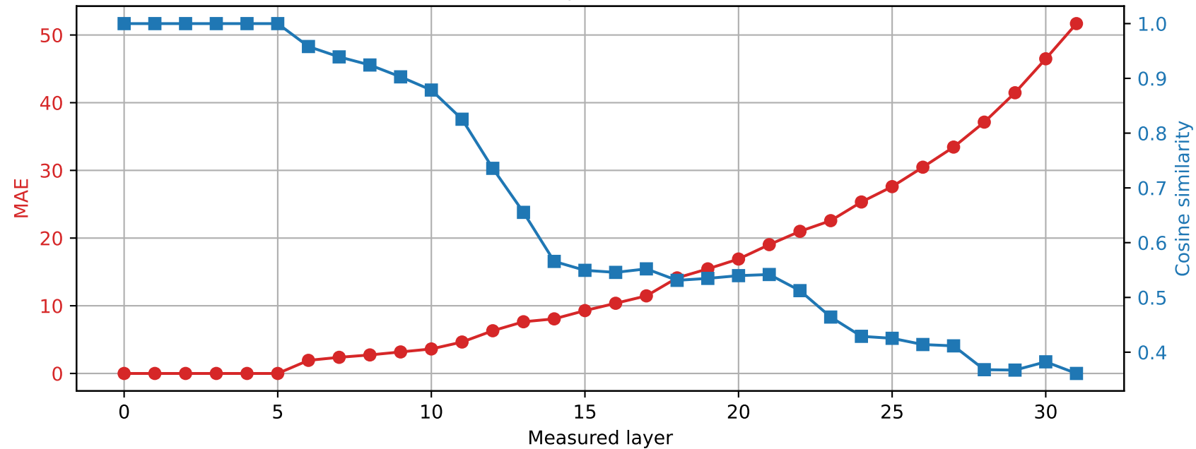
SmolLM2-360M | Prompt 1 Spared layer 5 | Hybrid vs quantized
