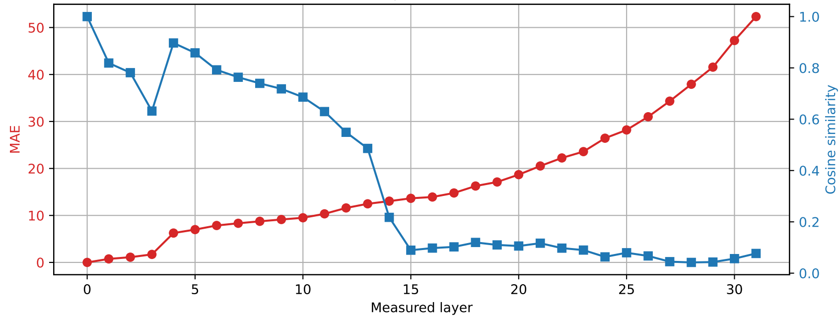
SmolLM2-360M | Prompt 1 Spared layer 14 | Hybrid vs unquantized
