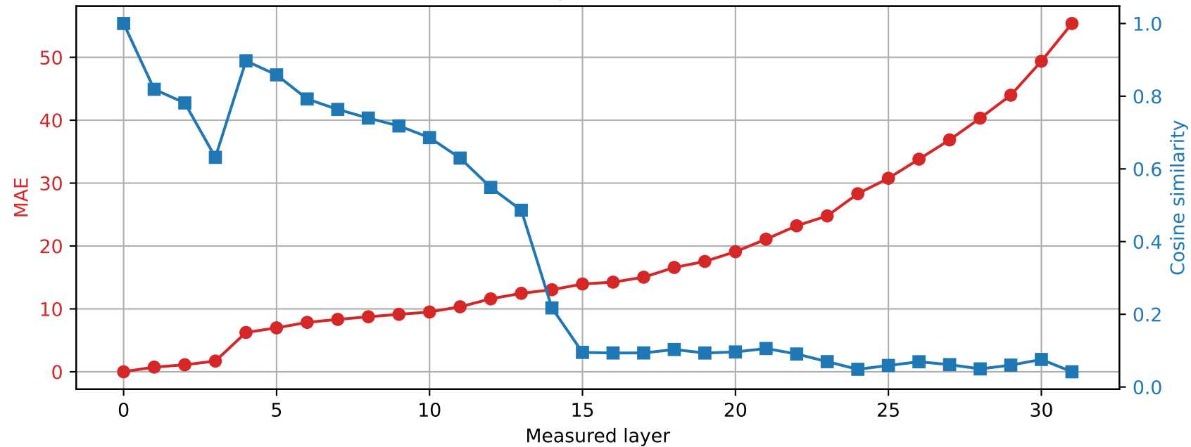
SmolLM2-360M | Prompt 1 Spared layer 15 | Hybrid vs unquantized
