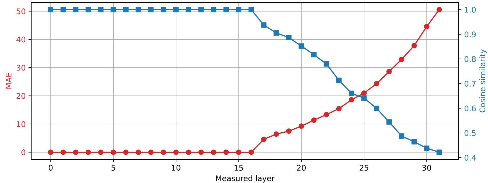
SmolLM2-360M | Prompt 1 Spared layer 16 | Hybrid vs quantized
