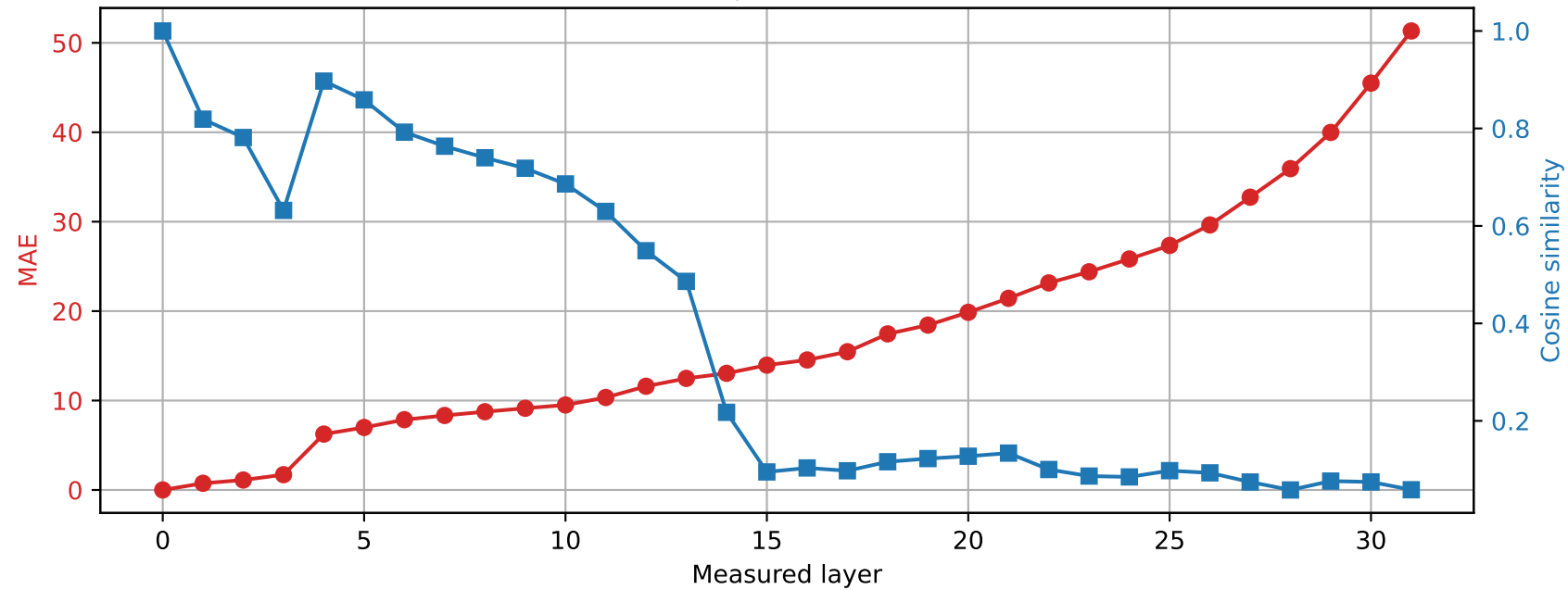
SmolLM2-360M | Prompt 1 Spared layer 23 | Hybrid vs unquantized
