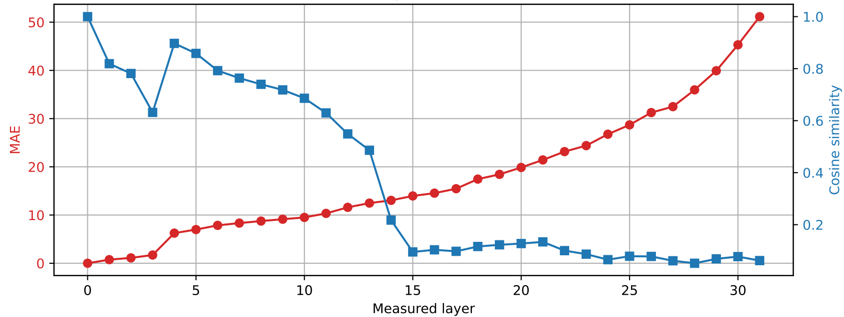
SmolLM2-360M | Prompt 1 Spared layer 26 | Hybrid vs unquantized
