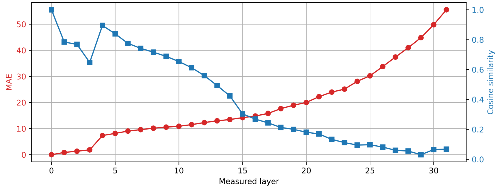
SmolLM2-360M | Prompt 2 Spared layer 2 | Hybrid vs unquantized
