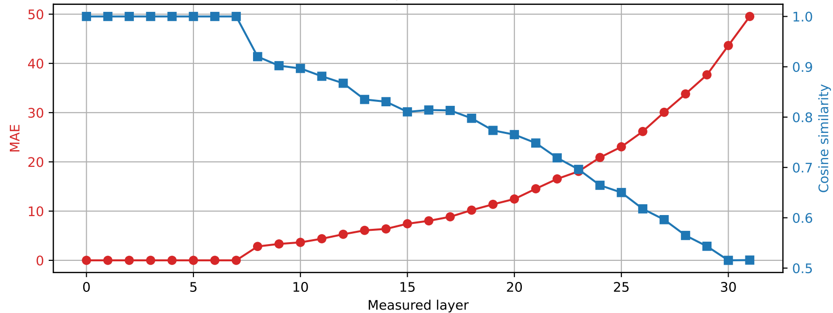
SmolLM2-360M | Prompt 2 Spared layer 7 | Hybrid vs quantized
