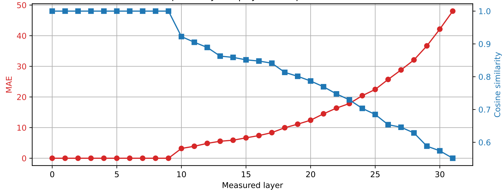
SmolLM2-360M | Prompt 2 Spared layer 9 | Hybrid vs quantized
