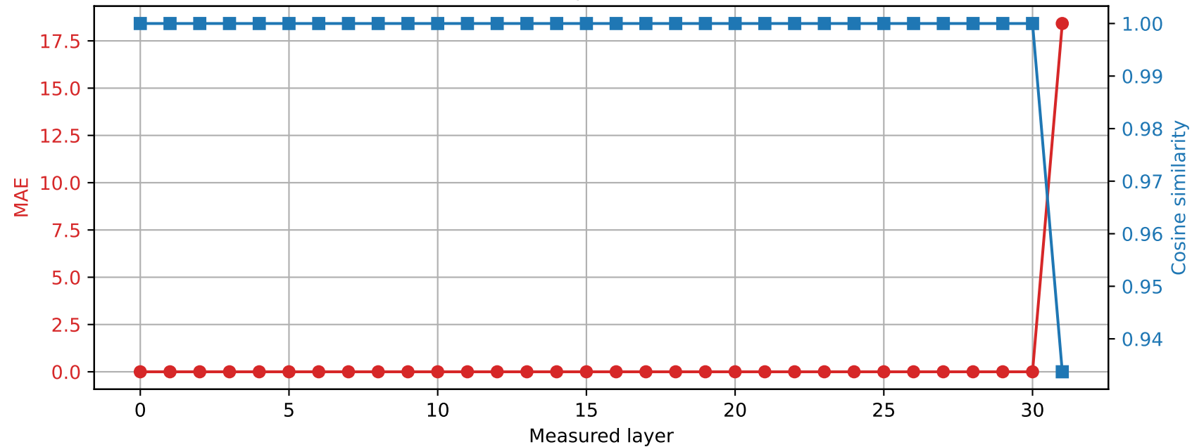
SmolLM2-360M | Prompt 2 Spared layer 30 | Hybrid vs quantized
