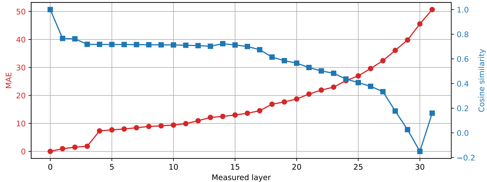
SmolLM2-360M | Prompt 3 Spared layer 2 | Hybrid vs unquantized
