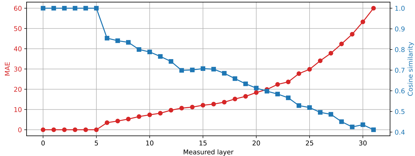
SmolLM2-360M | Prompt 3 Spared layer 5 | Hybrid vs quantized
