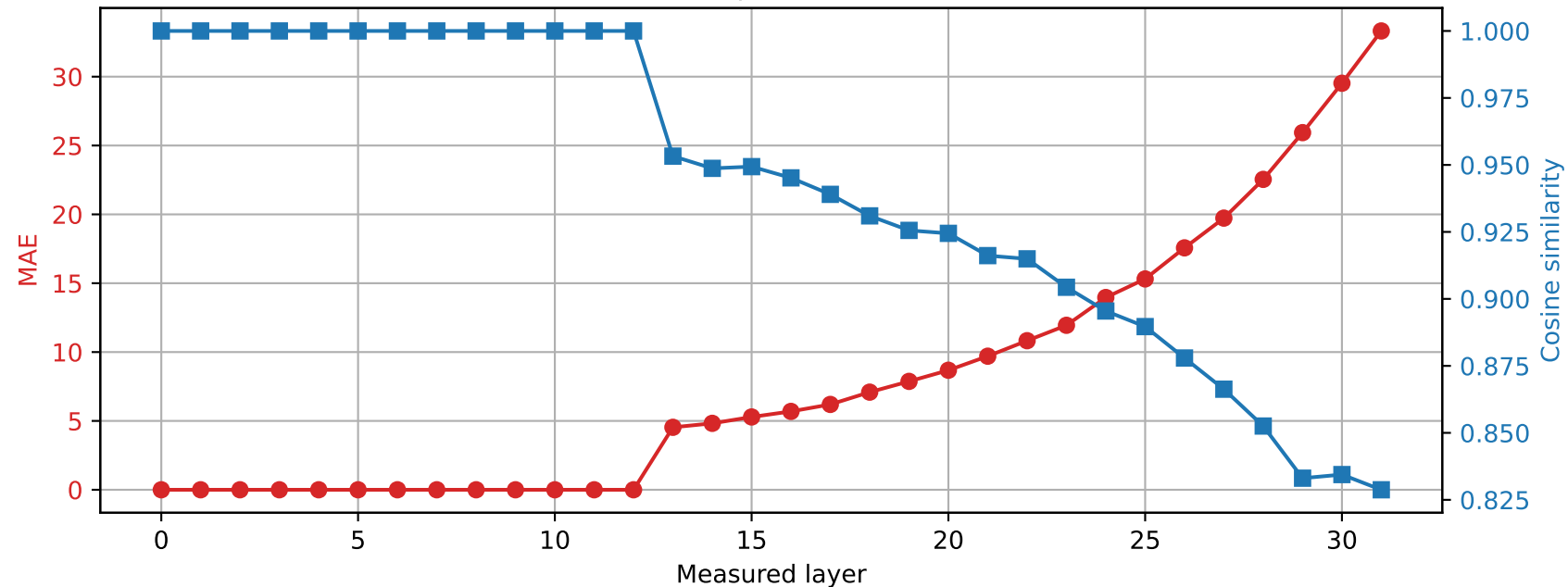
SmolLM2-360M | Prompt 3 Spared layer 12 | Hybrid vs quantized
