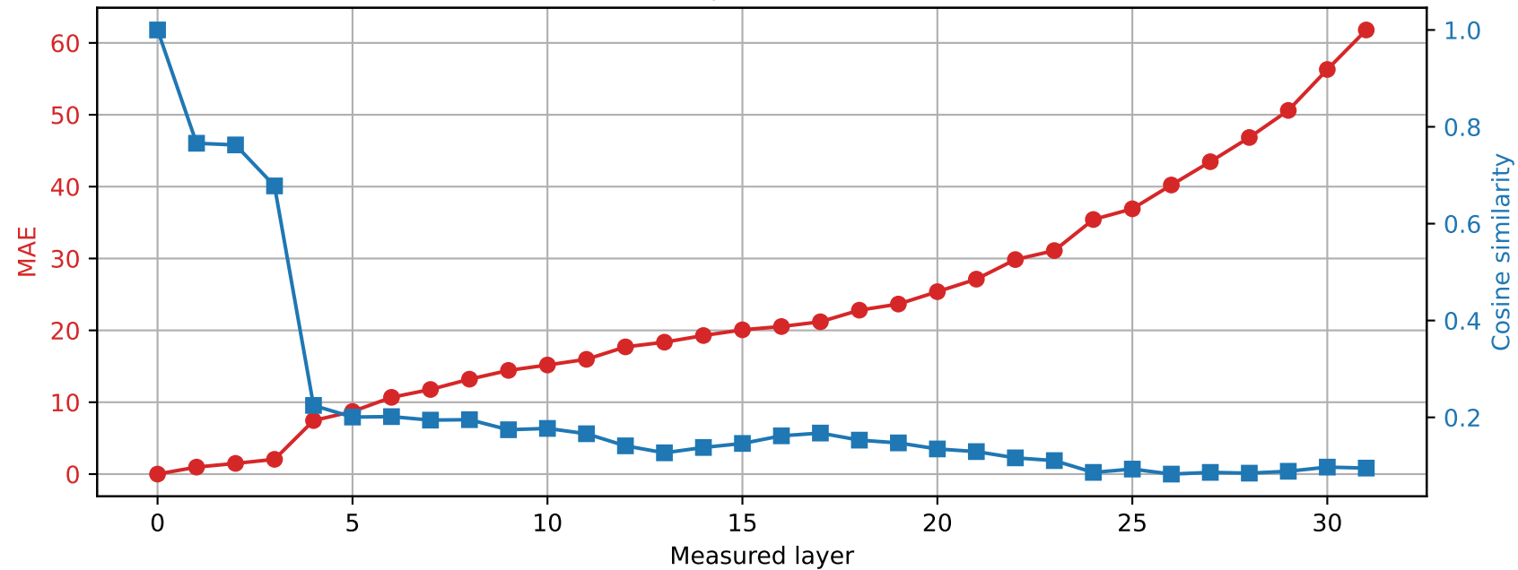
SmolLM2-360M | Prompt 3 Spared layer 13 | Hybrid vs unquantized
