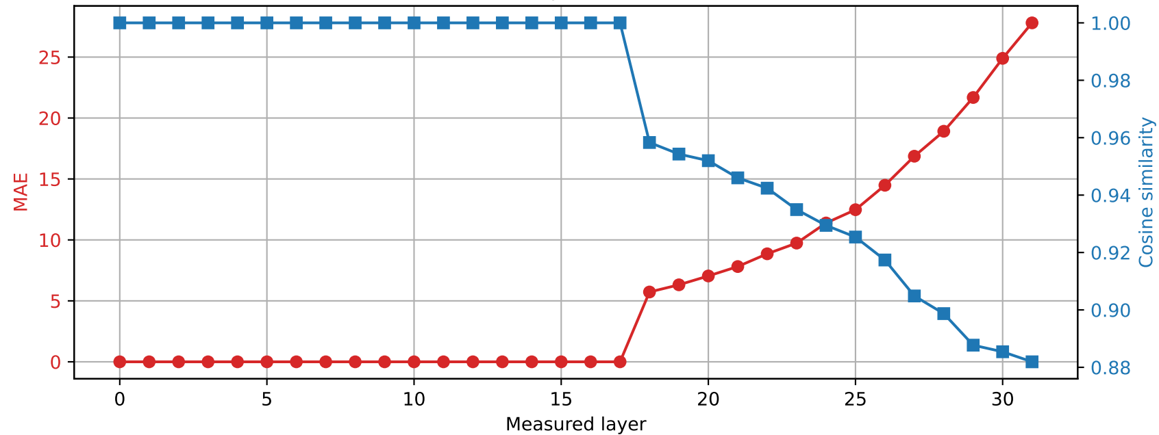
SmolLM2-360M | Prompt 3 Spared layer 17 | Hybrid vs quantized
