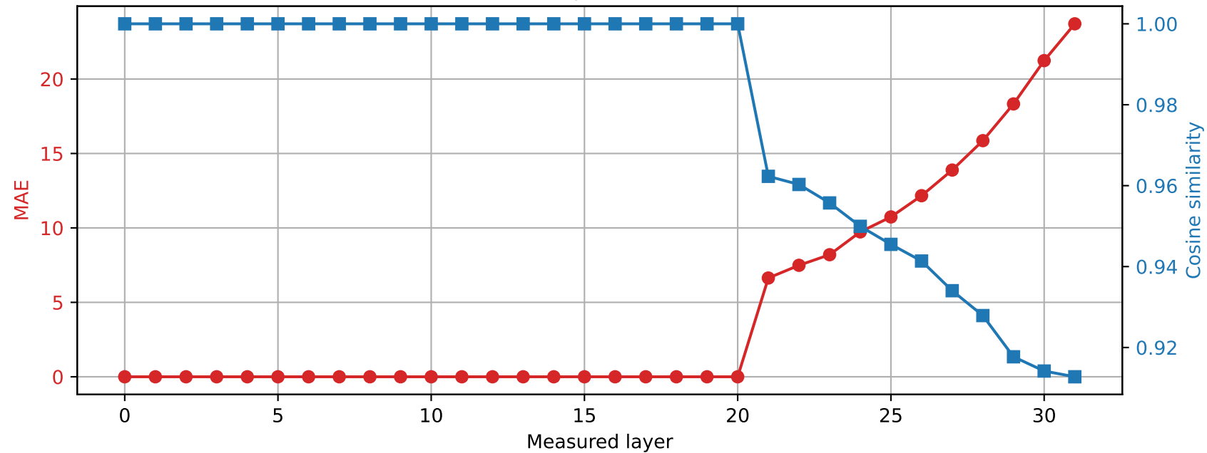
SmolLM2-360M | Prompt 3 Spared layer 20 | Hybrid vs quantized
