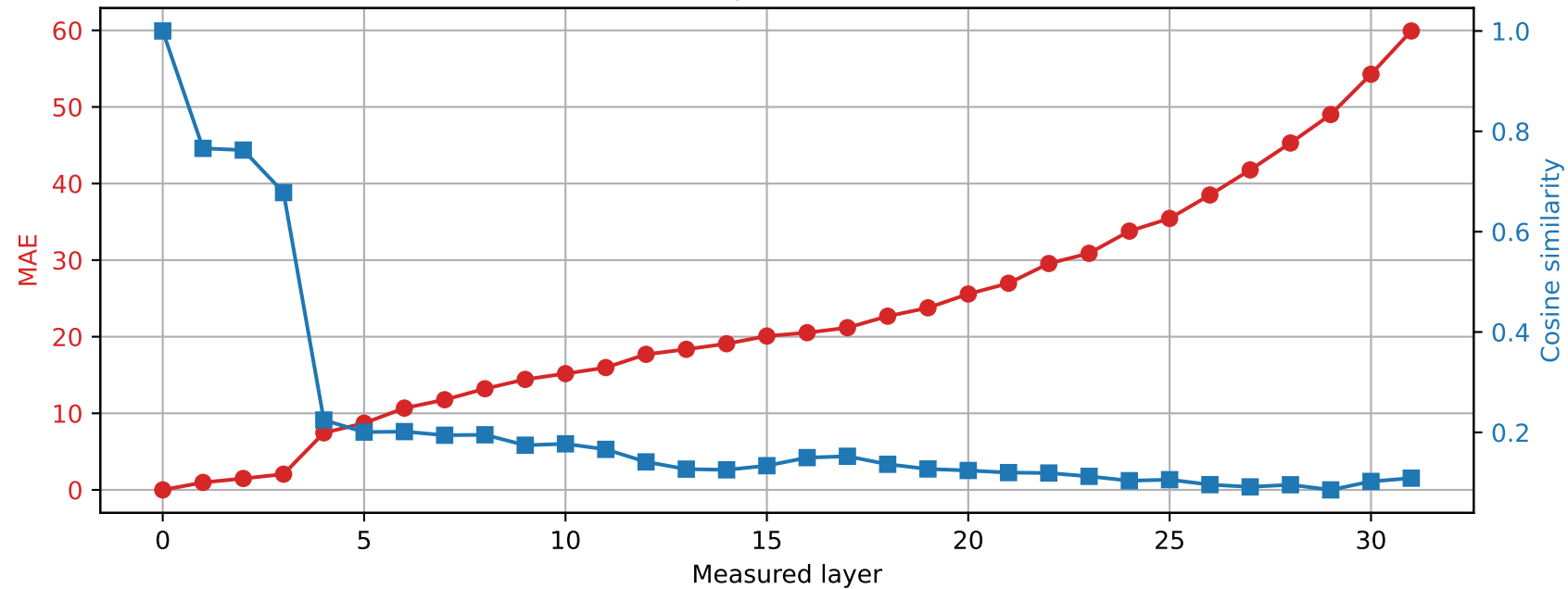
SmolLM2-360M | Prompt 3 Spared layer 23 | Hybrid vs unquantized
