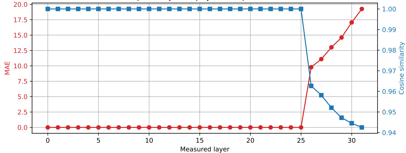
SmolLM2-360M | Prompt 3 Spared layer 25 | Hybrid vs quantized
